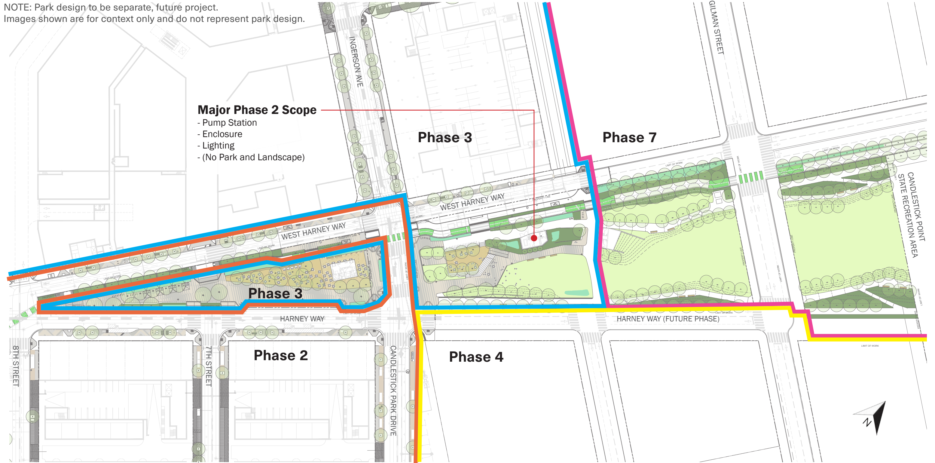
WILLIE MAYS PARK SITE PLAN (2016)
